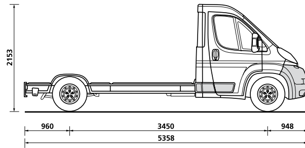
Plancher Cabine L2
