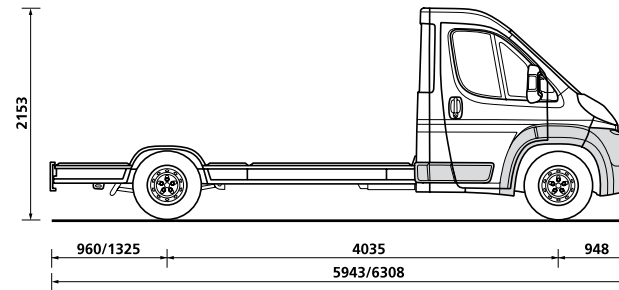
Plancher Cabine L3/L4
