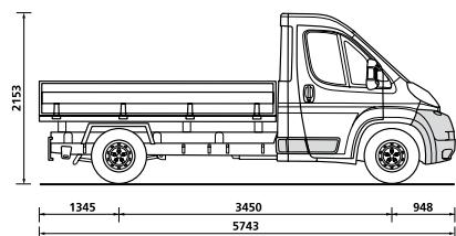
Plateaux Cabine L2
