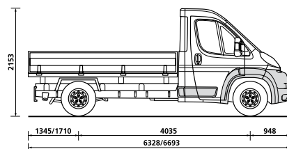
Plateaux Cabine L3/L4
