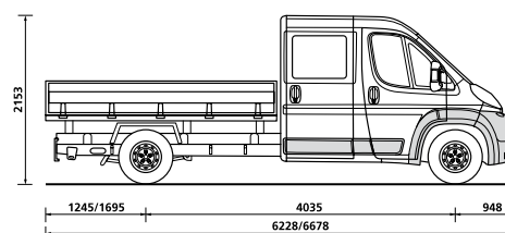
Plateaux Double Cabine L3/L4
